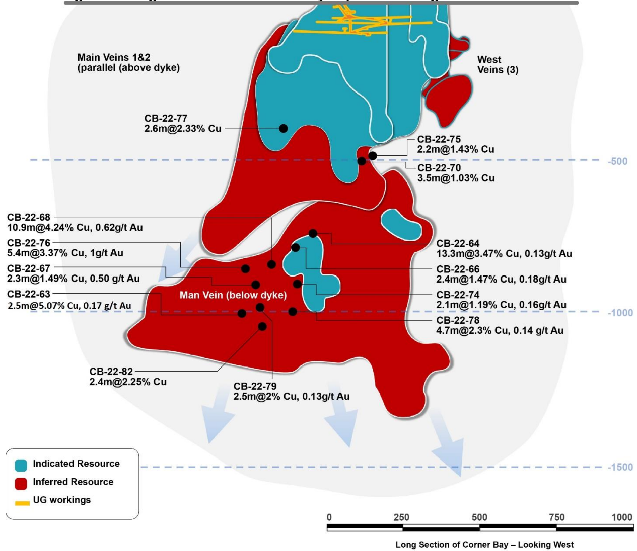
Figure 1. Long Section of the Corner Bay Deposit Showing the 2022 Drill Results
